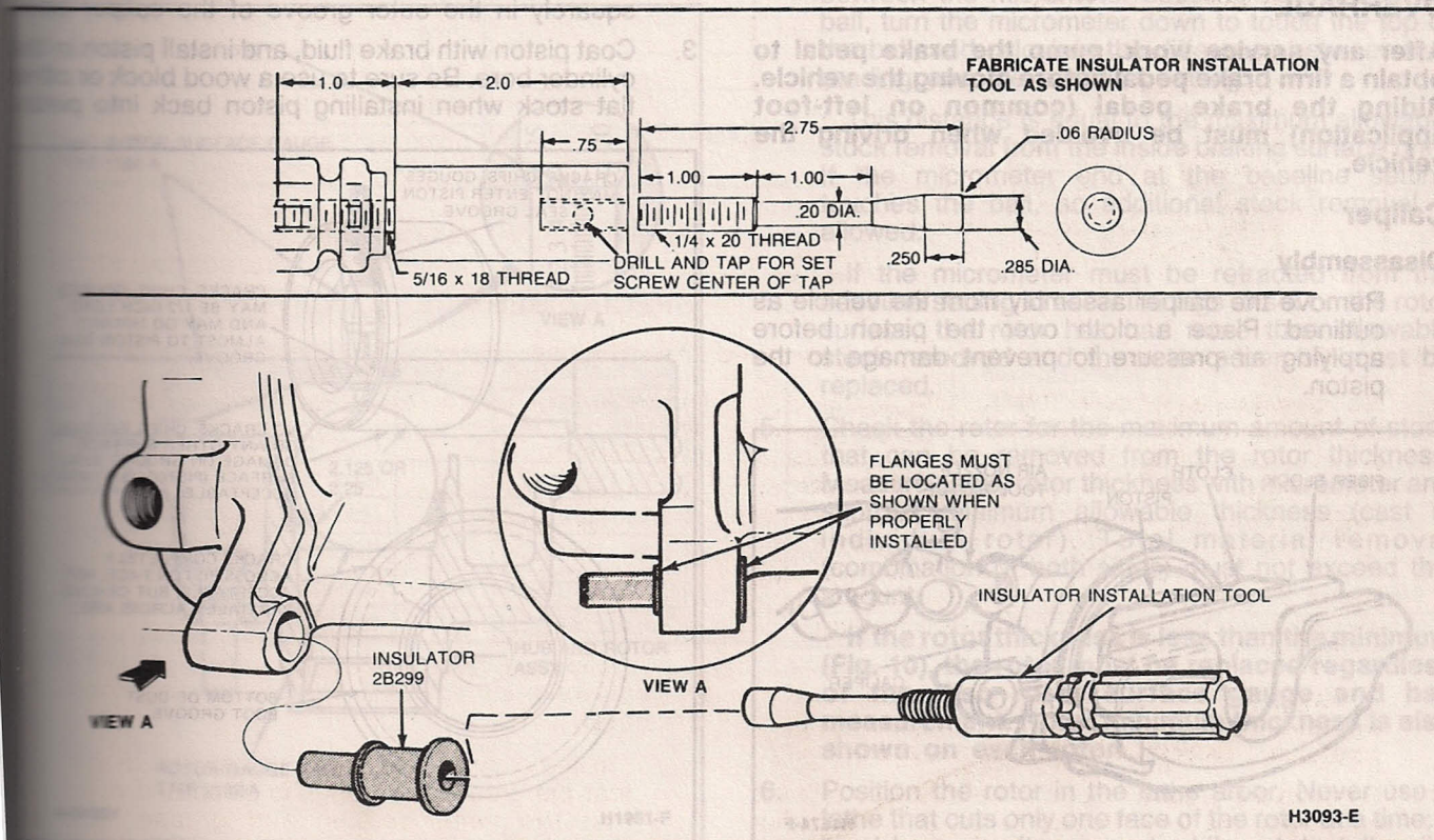
FIG. 7 Insulator and Sleeve Installation
