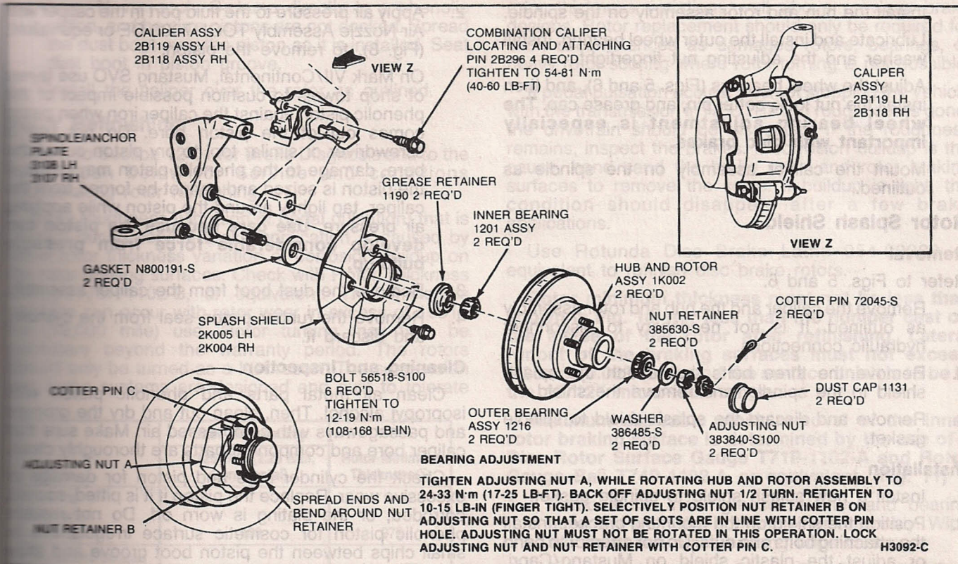
FIG. 6 Caliper, Shield, and Rotor Assemblies—Disc Brakes, Front—Mark VII/Continental, Mustang SVO
