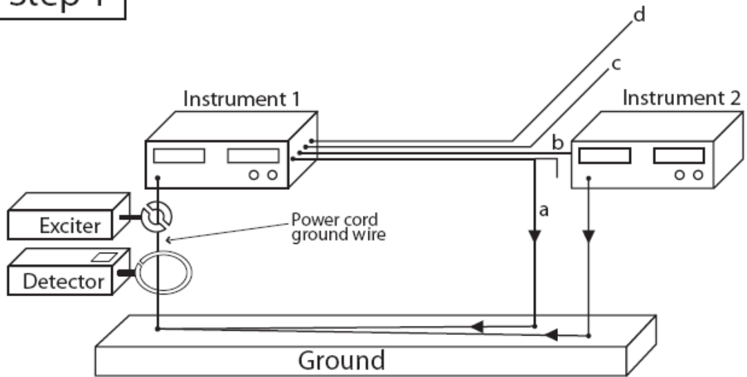
Figure 8 Step1: To check whether Instrument 1 has a ground loop, both Exciter and Detector are linked to power cord of Instrument 1. In this example there are ground loop paths through cables a and b. Cable a has accidental short to ground. All wires shown are ground or shield wires.
