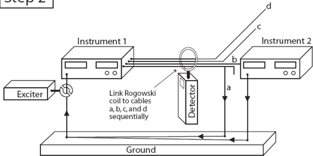
Figure 9 Step 2: The identity of the cable(s) involved in the ground loop is determined by linking the Detector Rogowski coil sequentially to cables a, b, c, and d. When the Rogowski coil links one or both of cables a and b, the Detector LED will illuminate indicating presence of ground loop current driven by Exciter. If the Rogowski coil links neither a nor b, then the indicator will not illuminate. The meter provides information on the relative amounts of ground loop current flowing in a and in b. All wires shown are ground or shield wires.
