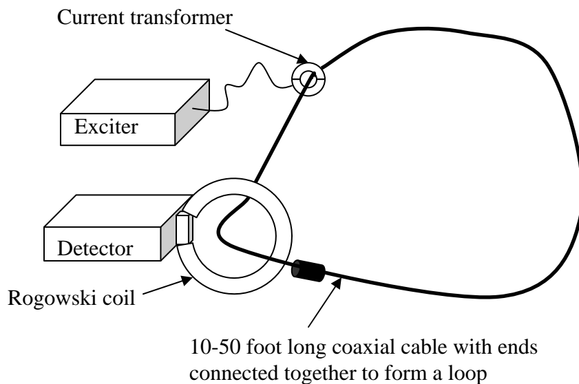
Figure 7. Basic setup: Exciter drives current in loop; Detector detects this current; loop must exist.
