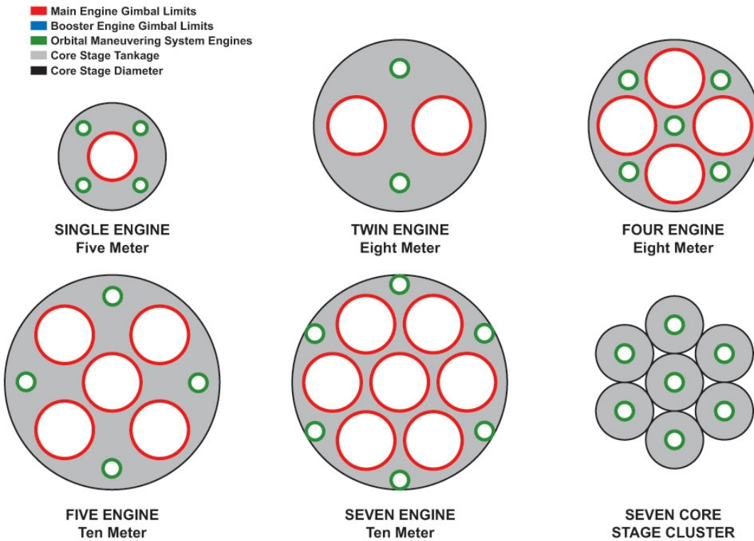
Figure 1. Five, Eight, and Ten Meter Launch Vehicle Engine Cluster Diagrams
